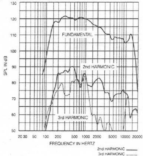
FIGURE 6 — Harmonic Distortion
