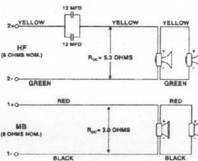
FIGURE 7 — Wiring Diagram
